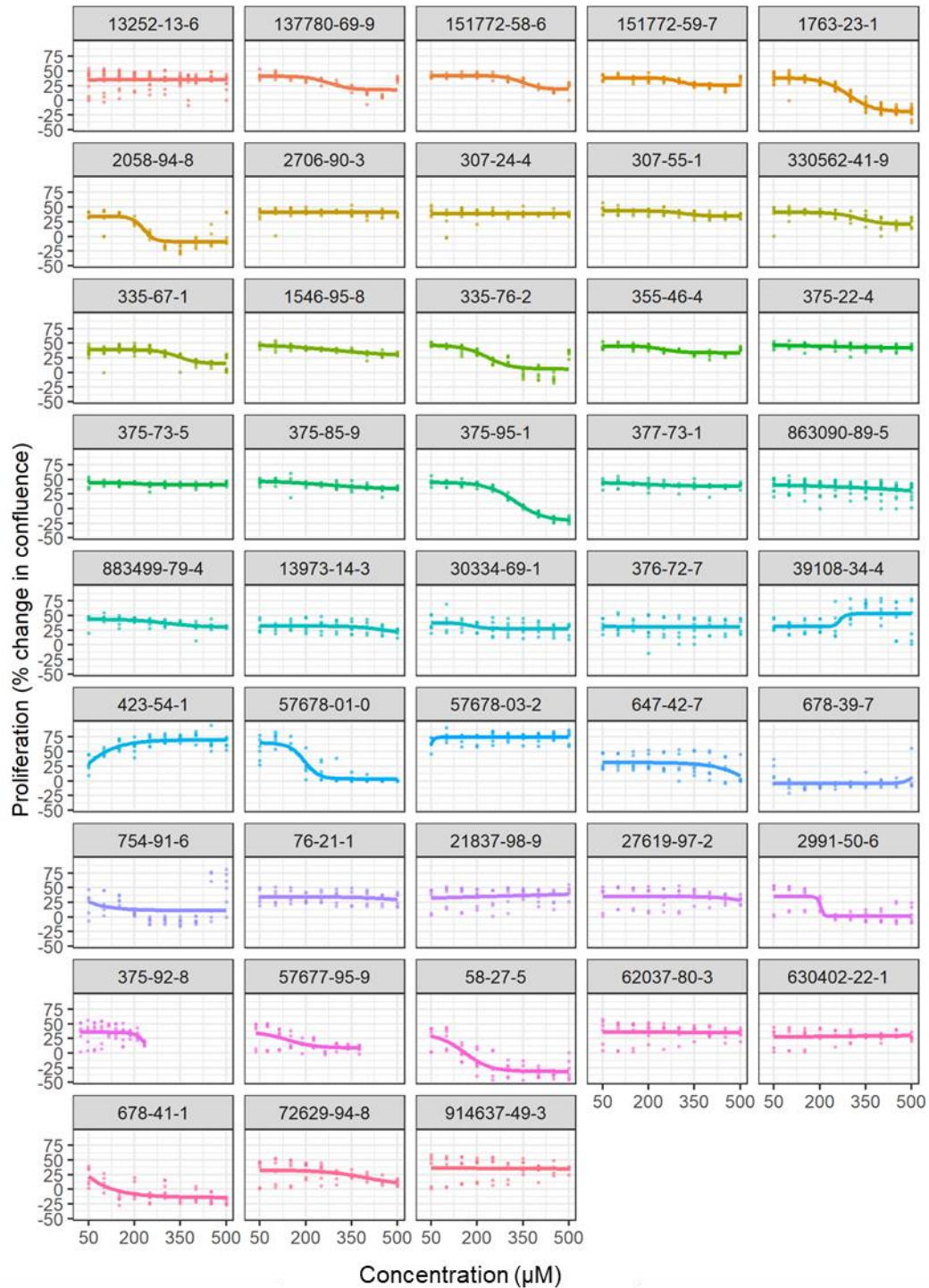
Supplementary Figure 5. Concentration-response model fits for cell proliferation after 24 hours exposure to PFAS. CAS numbers are shown in the grey header of individual plots. Data were fit to a four-parameter concentration-response model with no constraints and EC50 estimates were extracted. N = 3 biological replicates.
