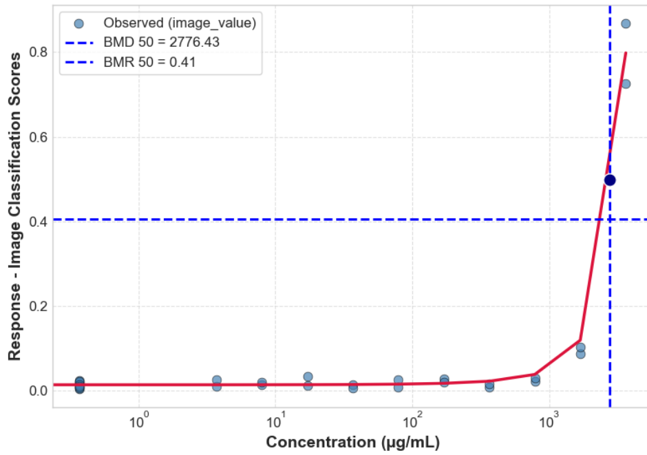
GBF-M HRG2DC CTG 24H 4_HRG2DC_P4_24H_REP3_CTG
