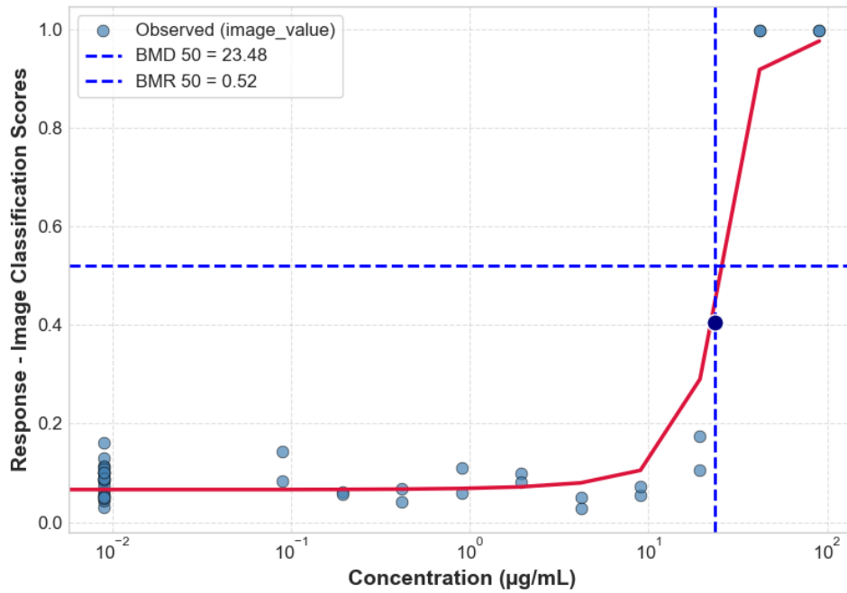
TBHP HRG2DC ROSGLO 24H 4_HRG2DC_P5_24H_REP2_ROSGLO
