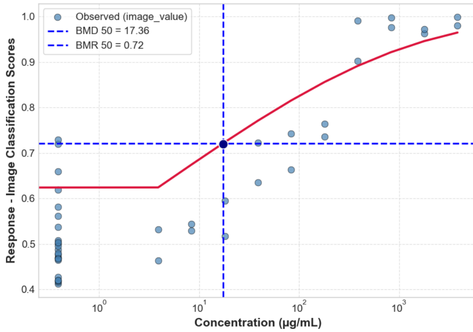
GBF-C HACAT CTG 24H 4_HACAT_P5_24H_REP2_CTG
