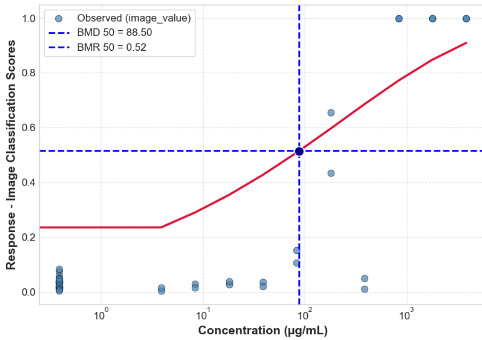
GBF-C HRG2DC CTG 24H 4_HRG2DC_P5_24H_REP3_CTG
