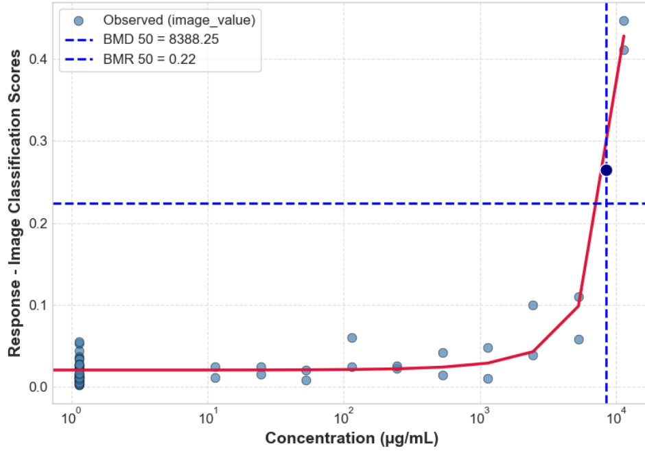
G-IPA HRG2DC CTG 24H 4_HRG2DC_P6_24H_REP3_CTG
