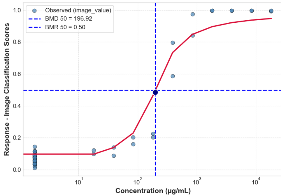
DIQUAT HRG2DC ROSGLO 24H 4_HRG2DC_P6_24H_REP2_ROSGLO
