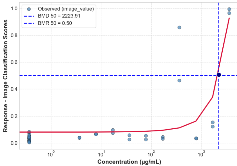
GBF-F HRG2DC CTG 24H 4_HRG2DC_P5_24H_REP3_CTG
