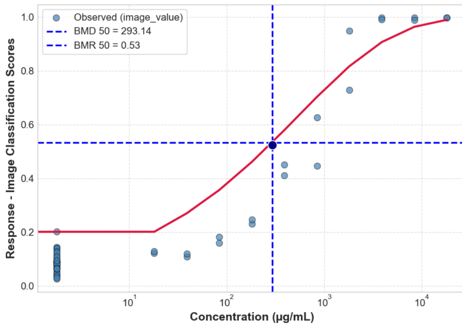
DIQUAT HRG2DC CTG 24H 4_HRG2DC_P6_24H_REP2_CTG
