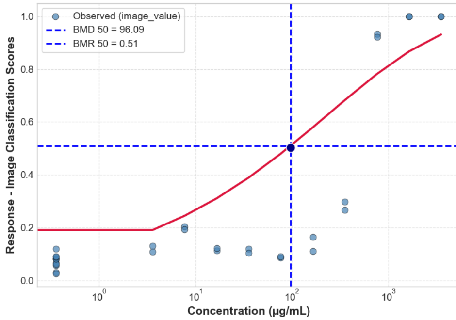
GBF-D HRG2DC CTG 24H 4_HRG2DC_P4_24H_REP2_CTG
