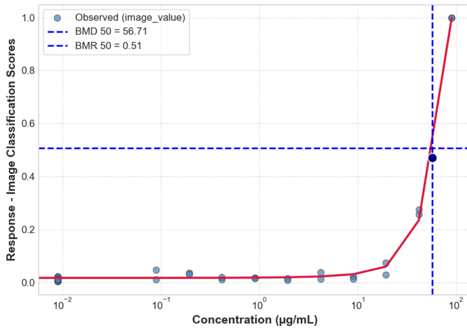
TBHP HRG2DC CTG 24H 4_HRG2DC_P4_24H_REP3_CTG
