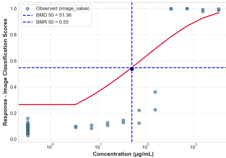
GBF-H HRG2DC ROSGLO 24H 4_HRG2DC_P5_24H_REP2_ROSGLO
