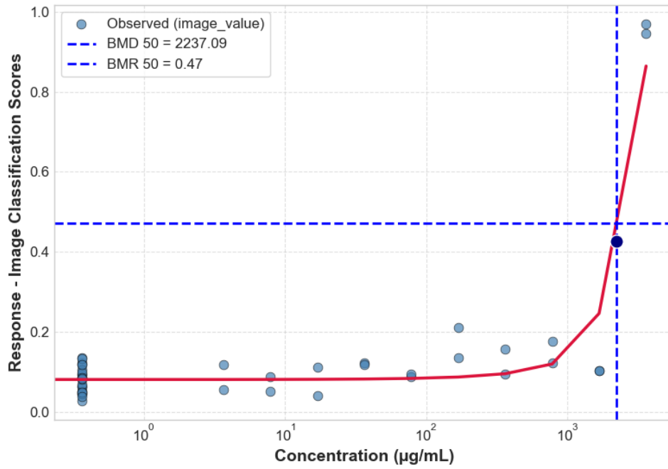
GBF-F HRG2DC CTG 24H 4_HRG2DC_P5_24H_REP2_CTG
