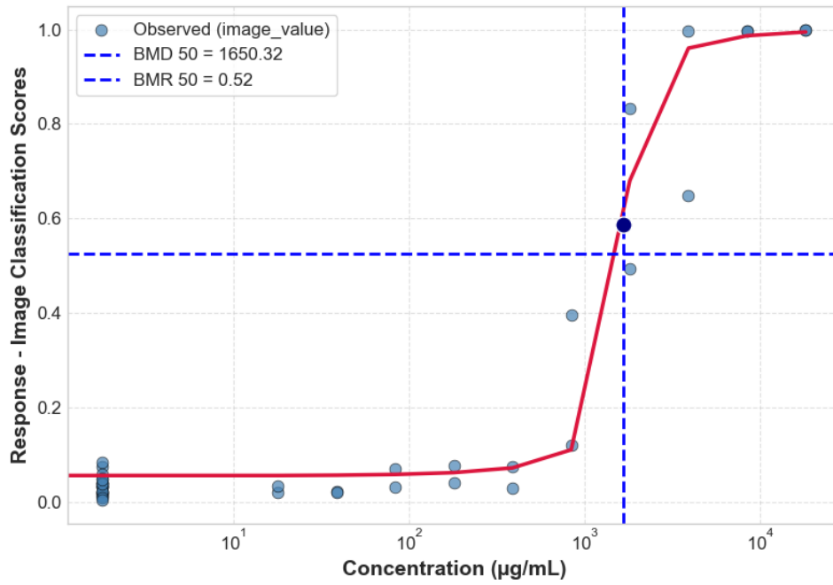
DIQUAT HRG2DC CTG 24H 4_HRG2DC_P5_24H_REP3_CTG
