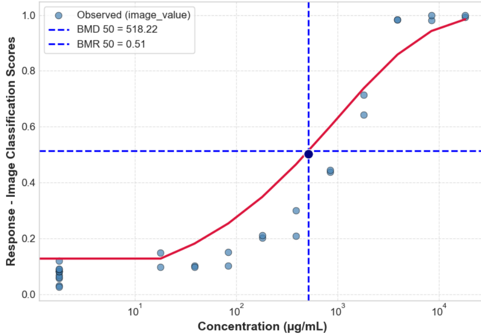
DIQUAT HRG2DC CTG 24H 4_HRG2DC_P4_24H_REP2_CTG
