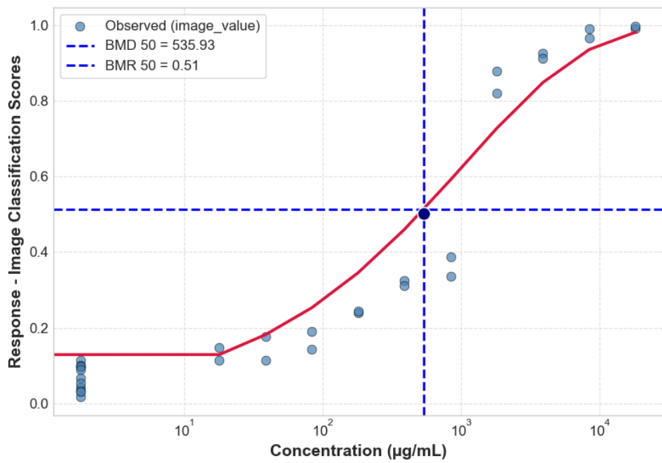
DIQUAT HRG2DC ROSGLO 24H 4_HRG2DC_P4_24H_REP2_ROSGLO
