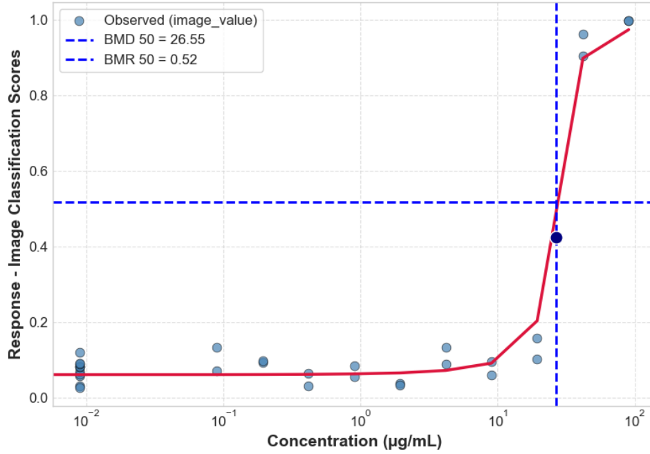
TBHP HRG2DC CTG 24H 4_HRG2DC_P4_24H_REP2_CTG
