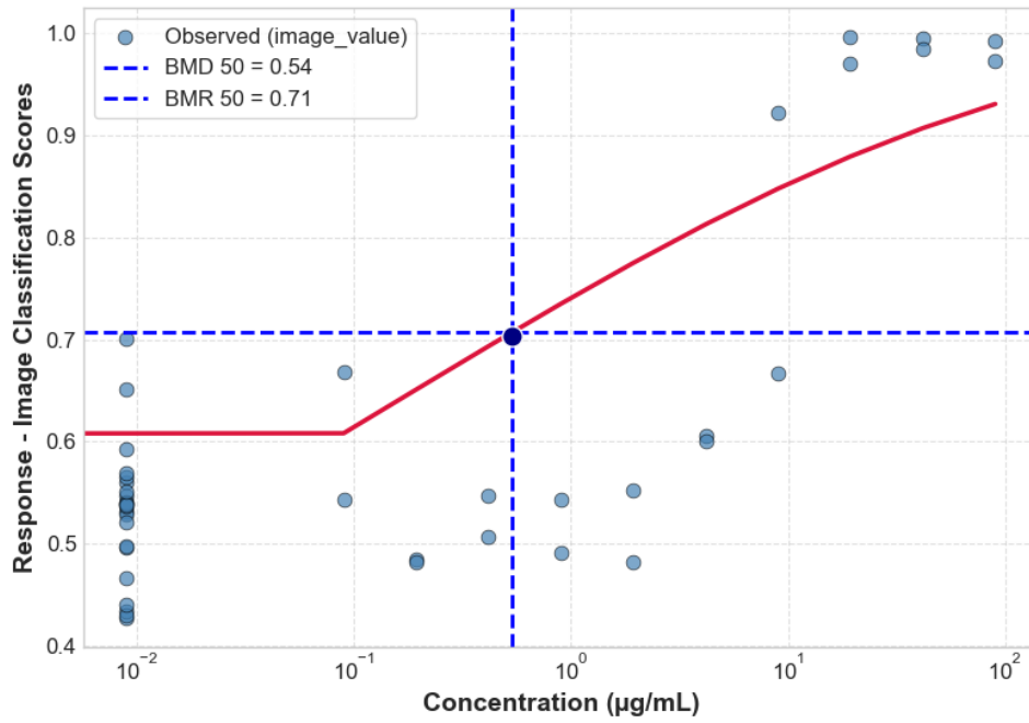
TBHP HACAT CTG 24H 4_HACAT_P5_24H_REP1_CTG
