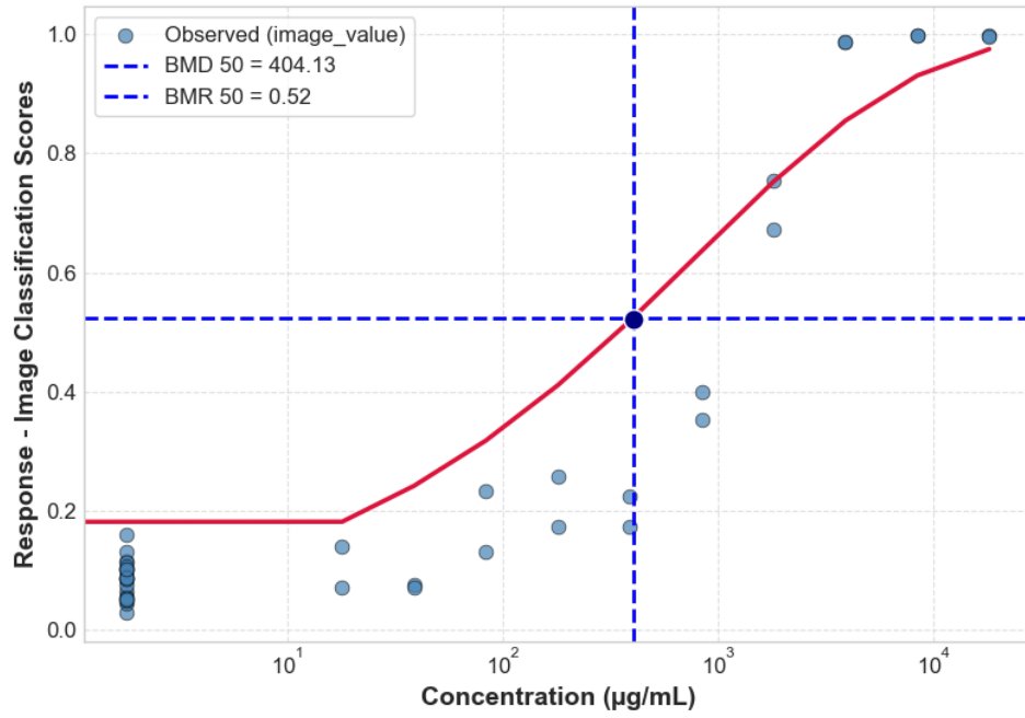
DIQUAT HRG2DC ROSGLO 24H 4_HRG2DC_P5_24H_REP2_ROSGLO
