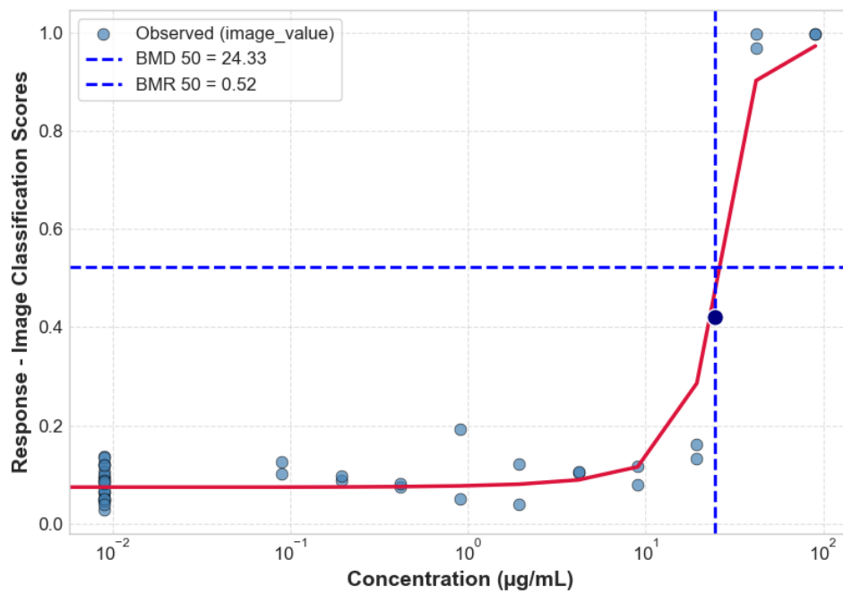
TBHP HRG2DC CTG 24H 4_HRG2DC_P5_24H_REP2_CTG
