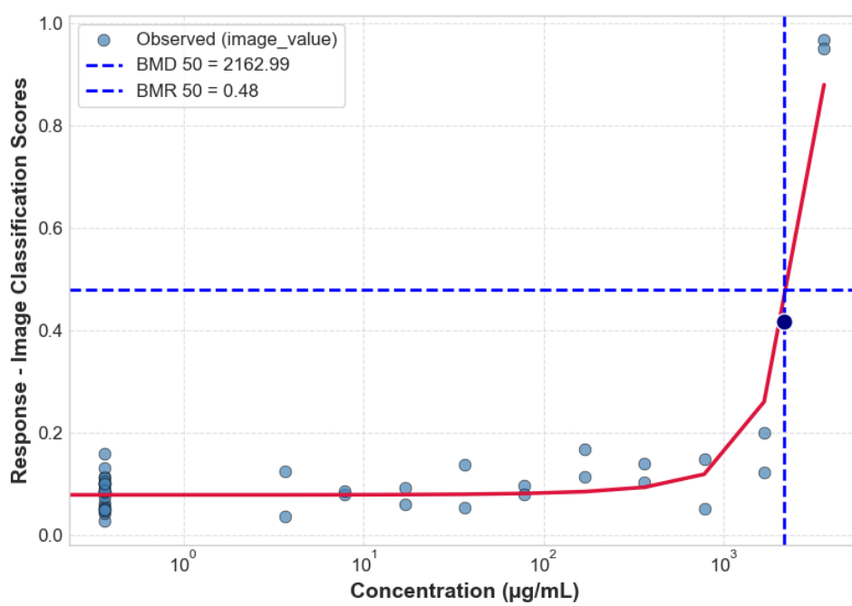
GBF-F HRG2DC ROSGLO 24H 4_HRG2DC_P5_24H_REP2_ROSGLO
