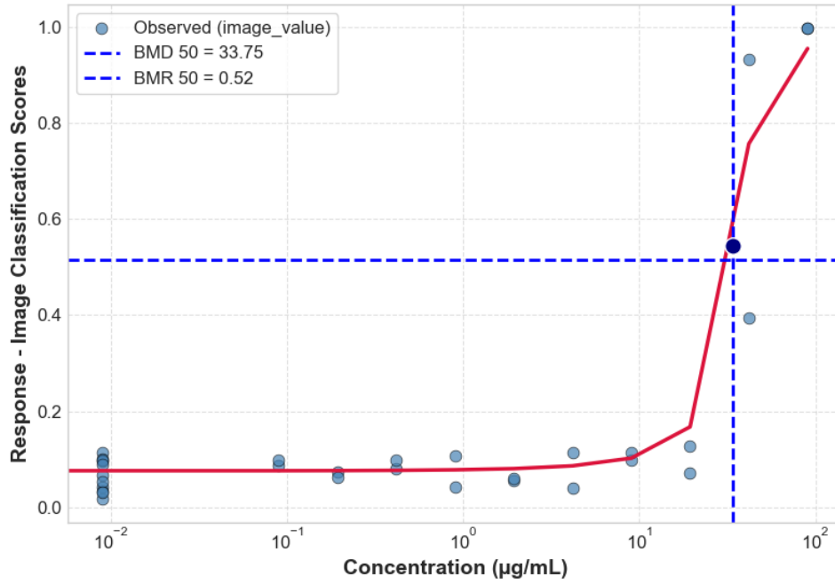
TBHP HRG2DC ROSGLO 24H 4_HRG2DC_P4_24H_REP2_ROSGLO
