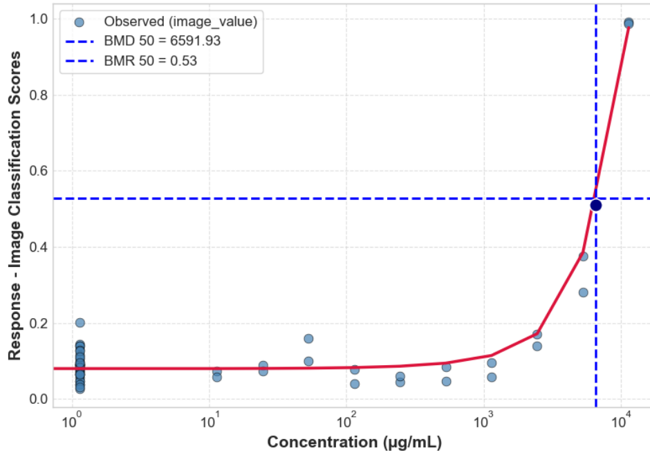
G-IPA HRG2DC CTG 24H 4_HRG2DC_P6_24H_REP2_CTG
