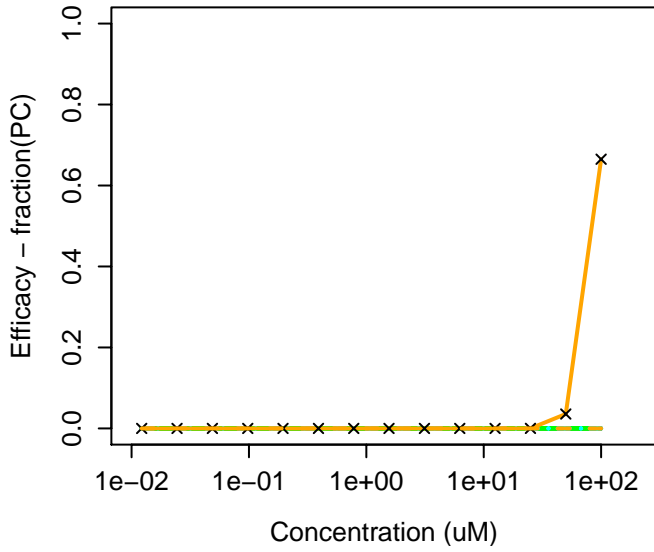
156-60-5 : (E)-1,2-Dichloroethylene
