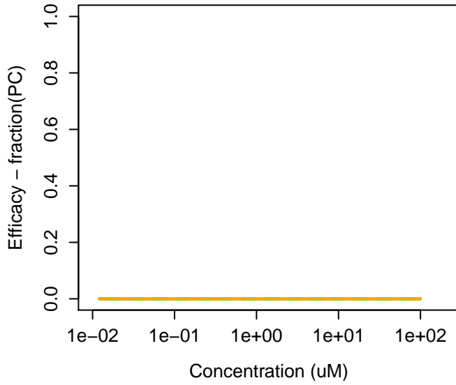
141-22-0 : (9Z,12R)-12-Hydroxyoctadec-9-enoic acid 141-22-0 : (9Z,12R)-12-Hydroxyoctadec-9-enoic acid Agonist: 0 Antagonist: 0
