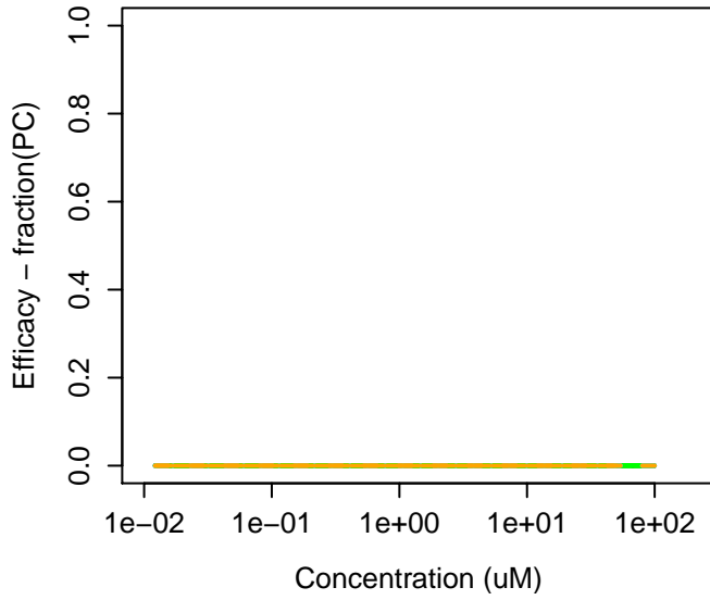
4712-55-4 : Diphenyl phosphite
