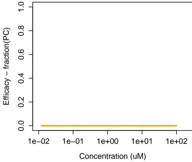
64359-81-5 : 4,5-Dichloro-2-octyl-3(2H)-isothiazolo[4,5-b]pyridin-6-amine Agonist: 0.0098 Antagonist: 0.094
