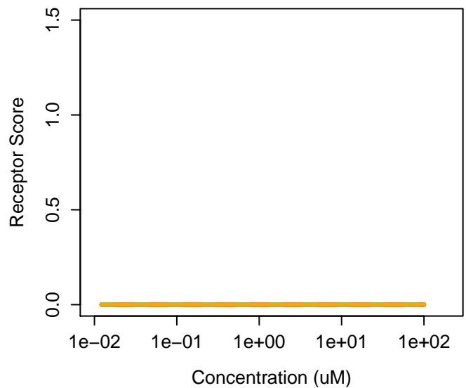
1072-15-7 : Sulfuric acid, monononyl ester, sodium 1072-15-7 : Sulfuric acid, monononyl ester, sodium Agonist: 0 Antagonist: 0
