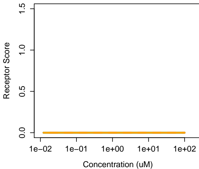
101-02-0 : Triphenyl phosphite Agonist: 0 Antagonist: 0
