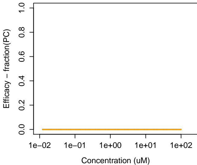
88-12-0 : N-Vinyl-2-pyrrolidone
