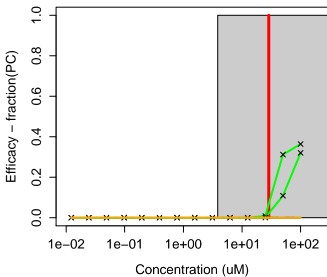
80-43-3 : Dicumyl peroxide
