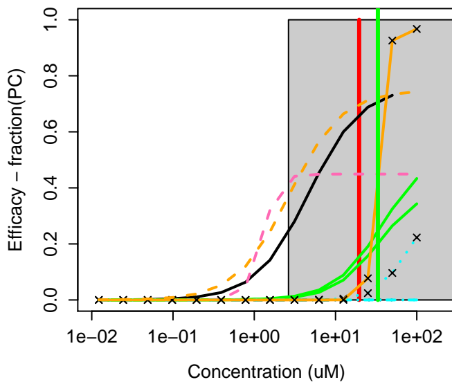
92-69-3 : 4-Phenylphenol
