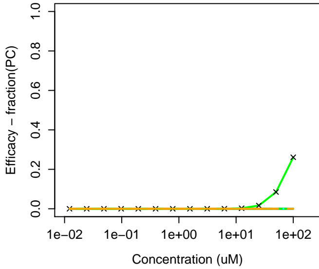
2144-53-8 : Tridecafluorohexylethyl methacrylate 2144-53-8 : Tridecafluorohexylethyl methacrylate Agonist: 0 Antagonist: 0
