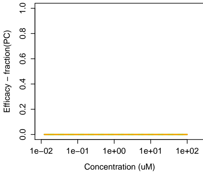
645-56-7 : 4-Propylphenol
