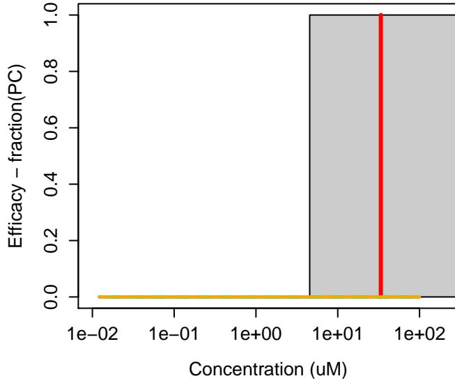
630-56-8 : Hydroxyprogesterone caproate
