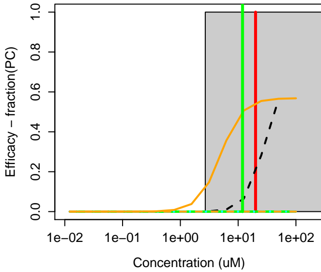
753-73-1 : Dimethyltin dichloride
