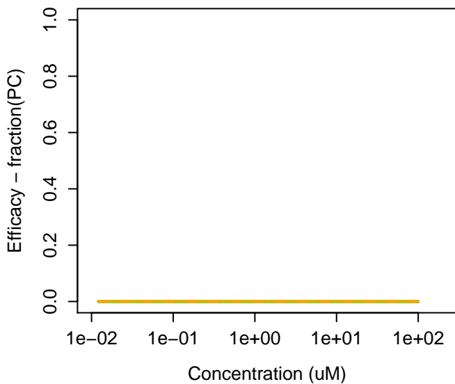
57-10-3 : Hexadecanoic acid
