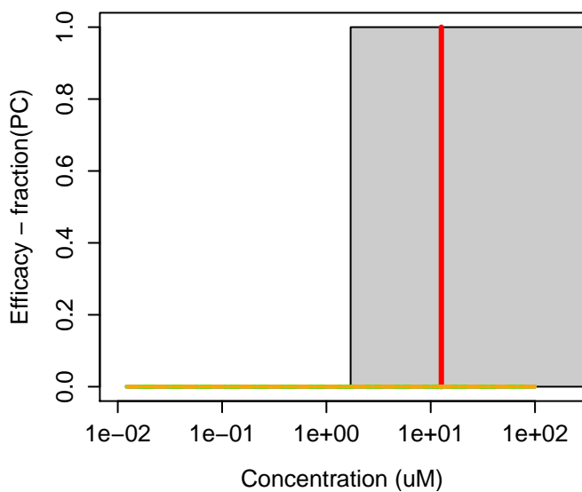
66332-96-5 : Flutolanil
