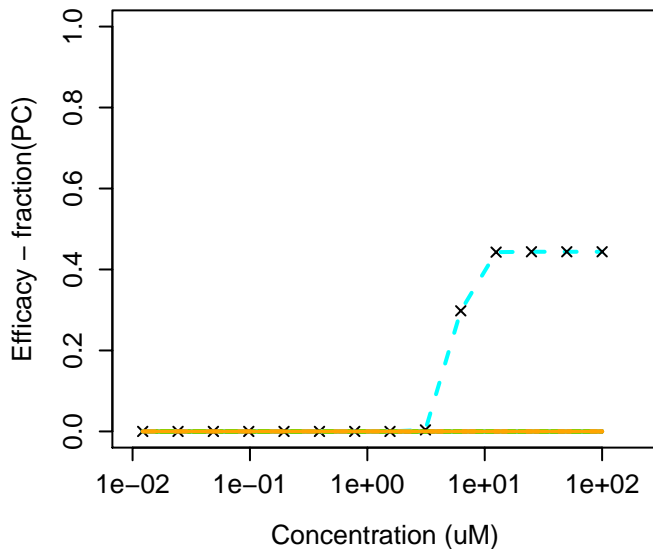
4376-18-5 : Monomethyl phthalate
