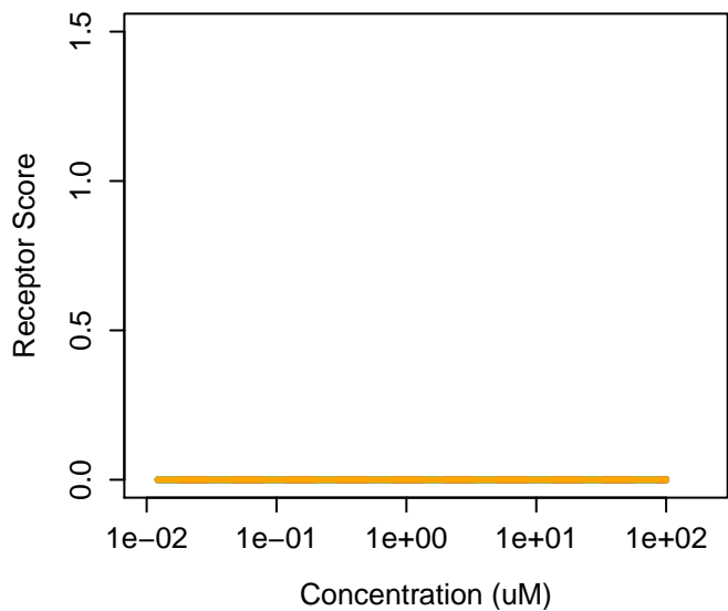
55589-62-3 : Acesulfame potassium Agonist: 0 Antagonist: 0
