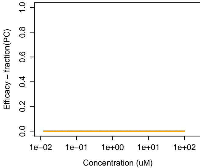
1072-15-7 : Sulfuric acid, monononyl ester, sodium 1072-15-7 : Sulfuric acid, monononyl ester, sodium Agonist: 0 Antagonist: 0
