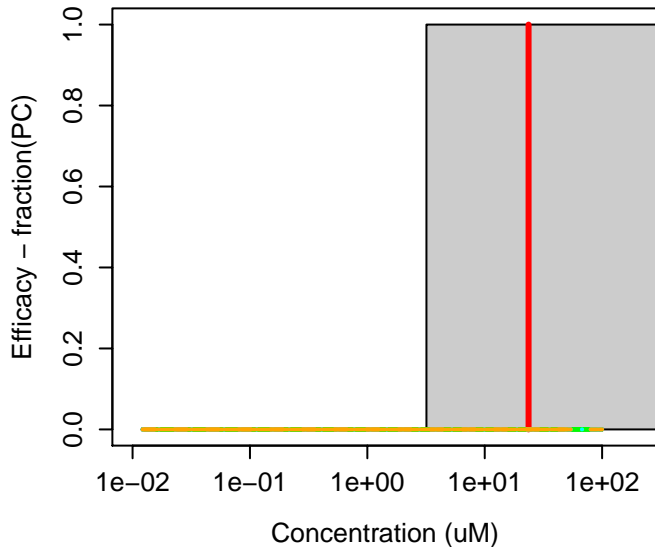
91-59-8 : 2-Naphthylamine
