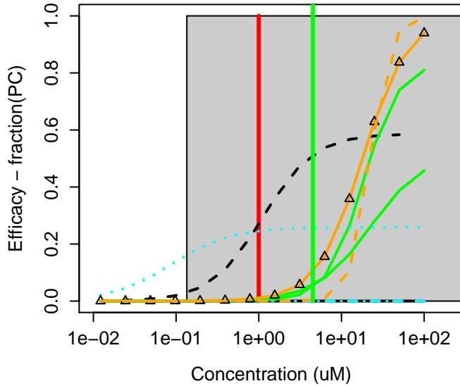
63-05-8 : 4-Androstene-3,17-dione
