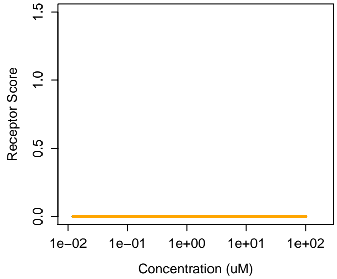
2144-53-8 : Tridecafluorohexylethyl methacrylate 2144-53-8 : Tridecafluorohexylethyl methacrylate Agonist: 0 Antagonist: 0
