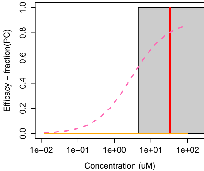
102-06-7 : 1,3-Diphenylguanidine
