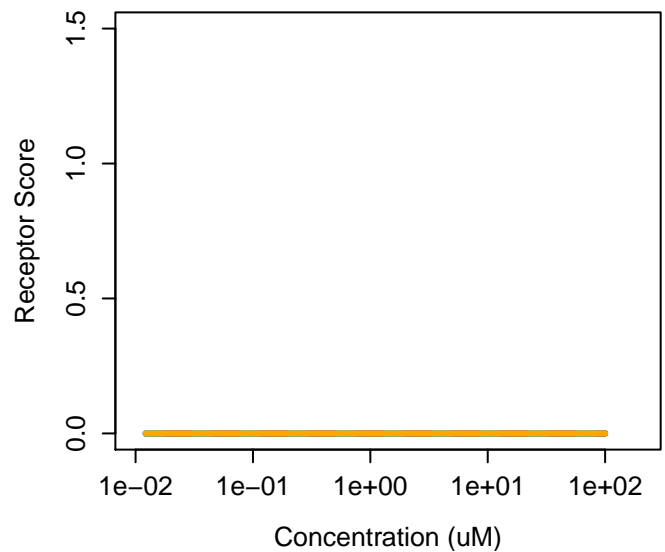
78-82-0 : 2-Methylpropanenitrile Agonist: 0 Antagonist: 0
