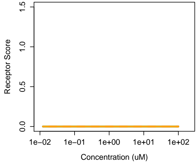
141-22-0 : (9Z,12R)-12-Hydroxyoctadec-9-enoic acid 141-22-0 : (9Z,12R)-12-Hydroxyoctadec-9-enoic acid Agonist: 0 Antagonist: 0
