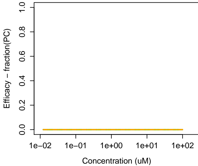
1024-57-3 : Heptachlor epoxide
