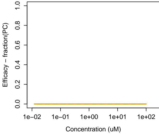
57-97-6 : 7,12-Dimethylbenz(a)anthracene
