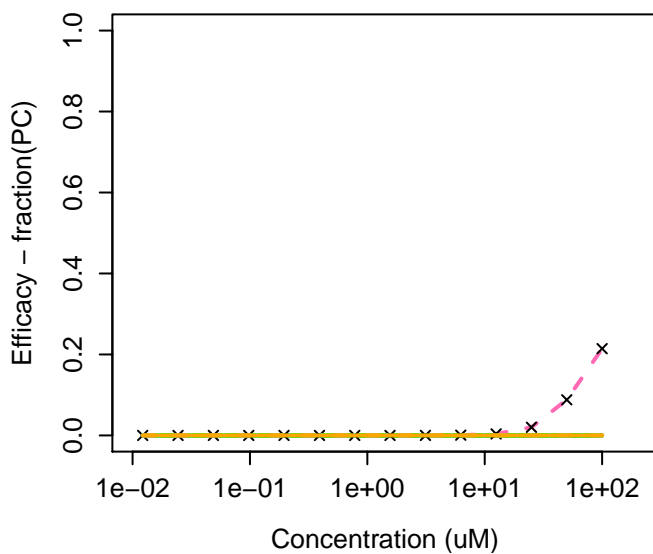
89-72-5 : 2-(Butan-2-yl)phenol
