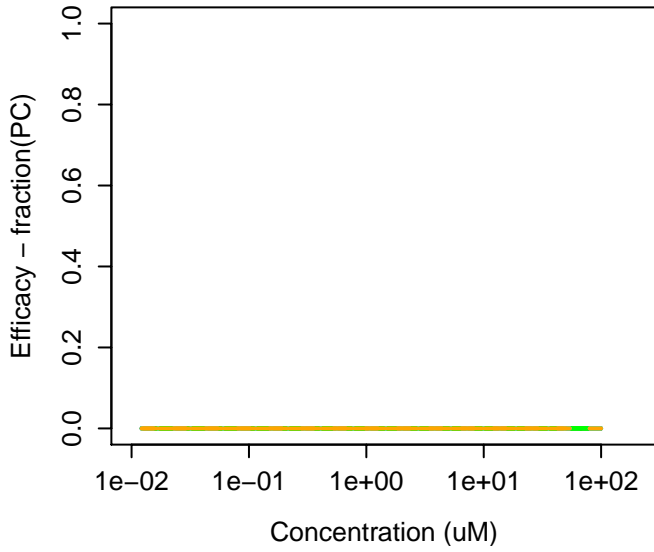
57-09-0 : Hexadecyltrimethylammonium bromid
