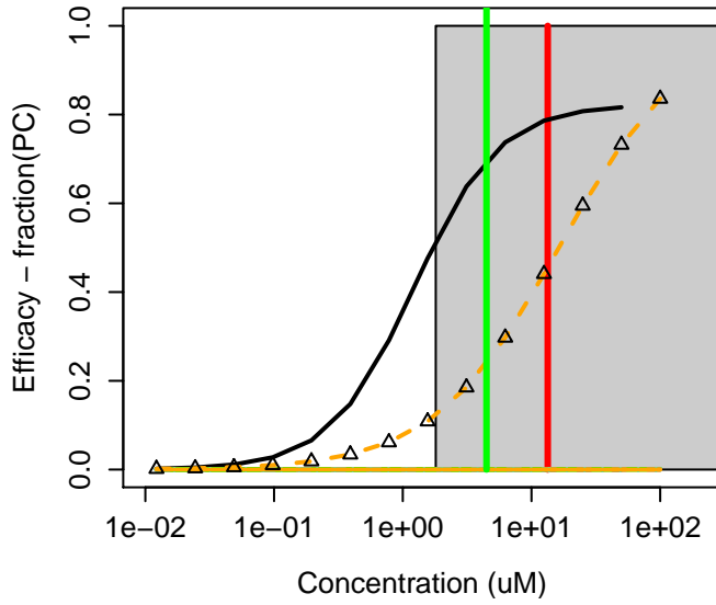
298-02-2 : Phorate
