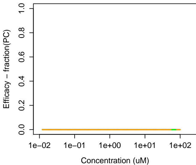
119-36-8 : Methyl salicylate
