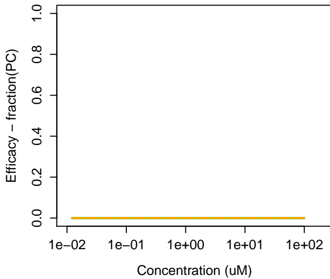
118-79-6 : 2,4,6-Tribromophenol
