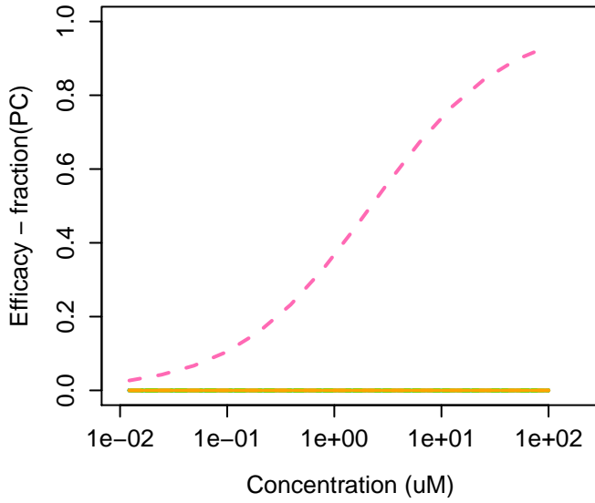
107-75-5 : 7-Hydroxy-3,7-dimethyloctanal
