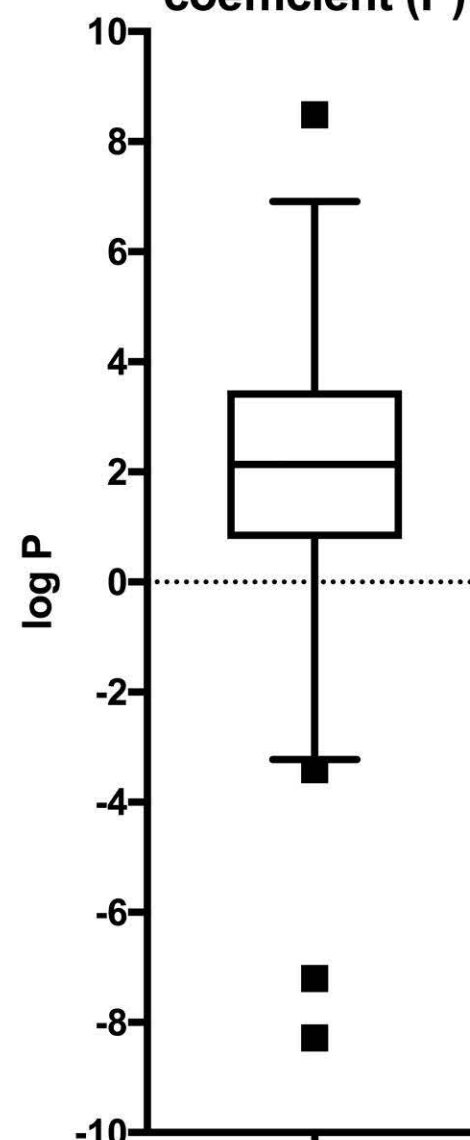
octanol-water partition coefficient (P)
