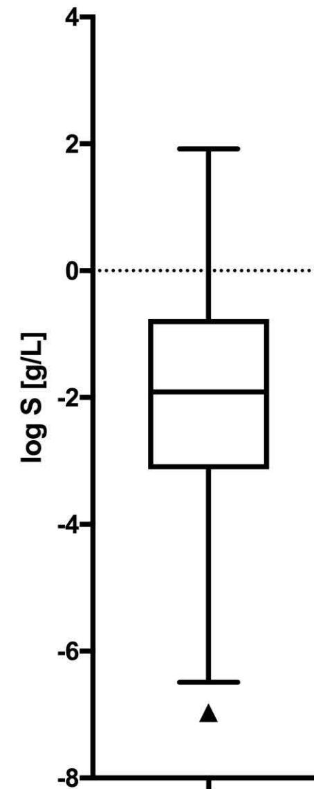
water solubility (S)
