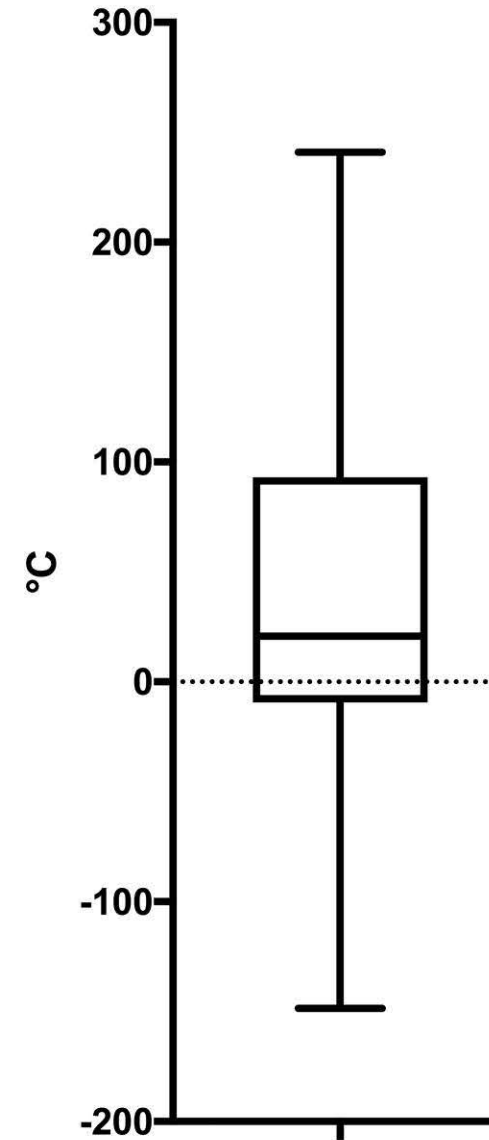
melting point (MP)
