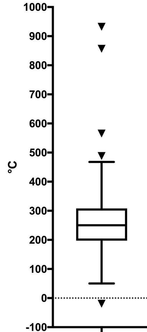
boiling point (BP)
