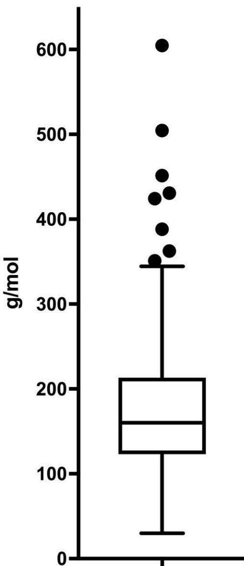
molecular weight (MW)
